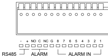
[Fig. 5-7 Alarm Output]
